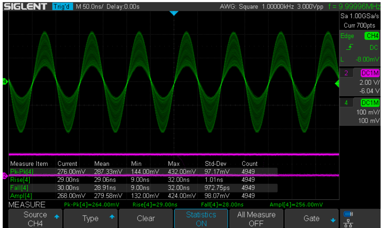
Sine_10MHz_AM1kHz_50%_M50ns_Dots
